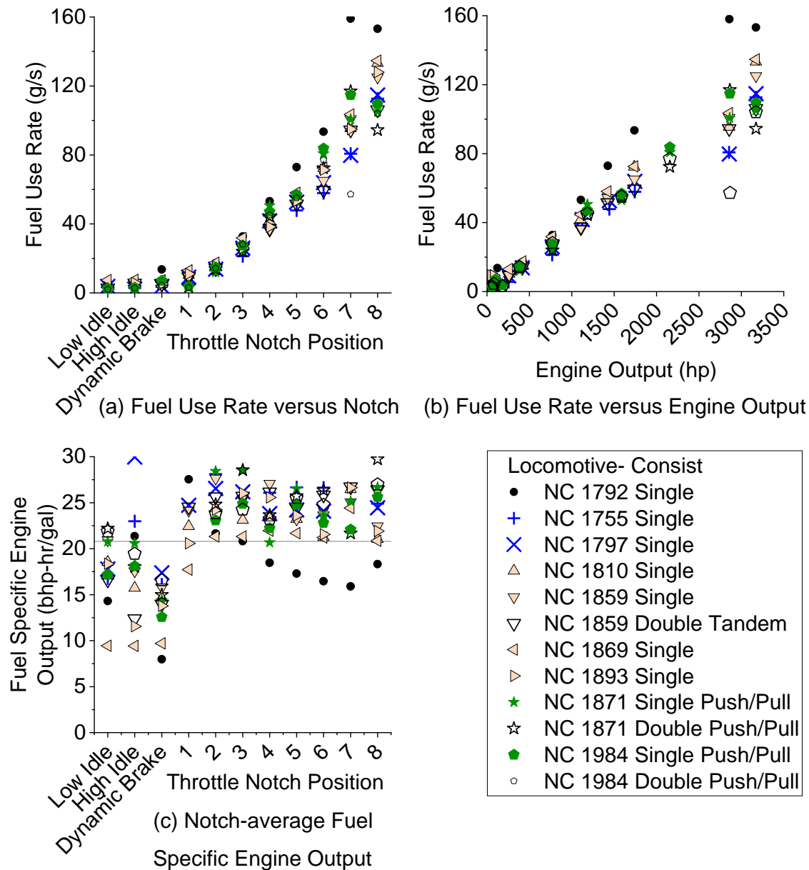
FIGURE 4-8. Steady-State based Notch-average Fuel Use Rates and Fuel Specific Engine Output for the Most Recent Over-the-rail Measurement of the Prime Mover Engines of all NCDOT Locomotives Operated on Ultra-low Sulfur Diesel: (a) Notch-average Fuel Use Rate versus Notch Position; (b) Notch-average Fuel Use Rate versus Engine Output; and (c) Notch-average Fuel Specific Engine Output.
