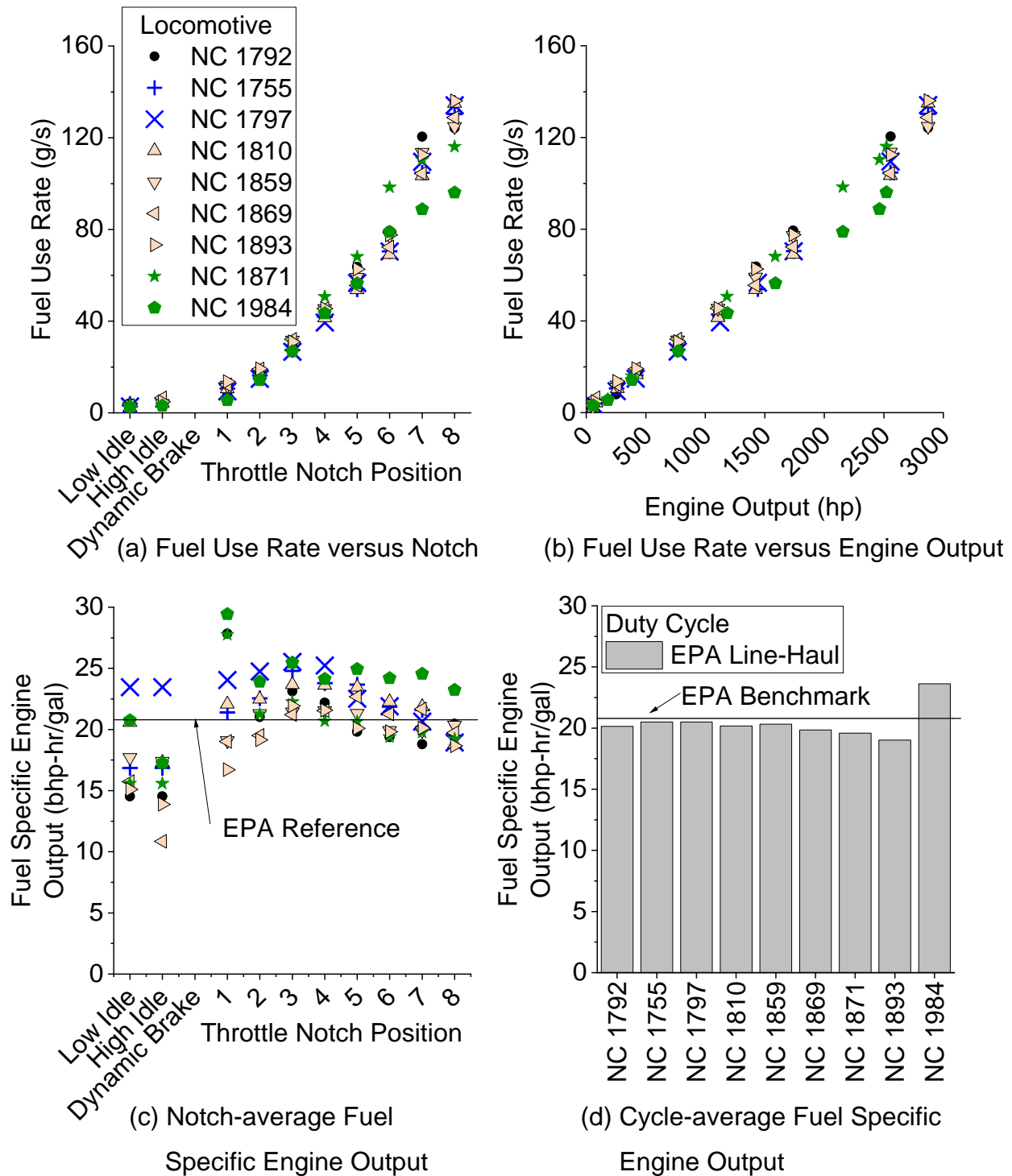
FIGURE 3-4. Notch-average Fuel Use Rates and Fuel Specific Engine Output for the Most Recent Rail Yard Measurement of the Prime Mover Engines of all NCDOT Locomotives Operated on Ultra-low Sulfur Diesel: (a) Notch-average Fuel Use Rate versus Notch Position; (b) Notch-average Fuel Use Rate versus Engine Output; (c) Notch-average Fuel Specific Engine Output; and (d) EPA Line-haul Cycle-average Fuel Specific Engine Output
