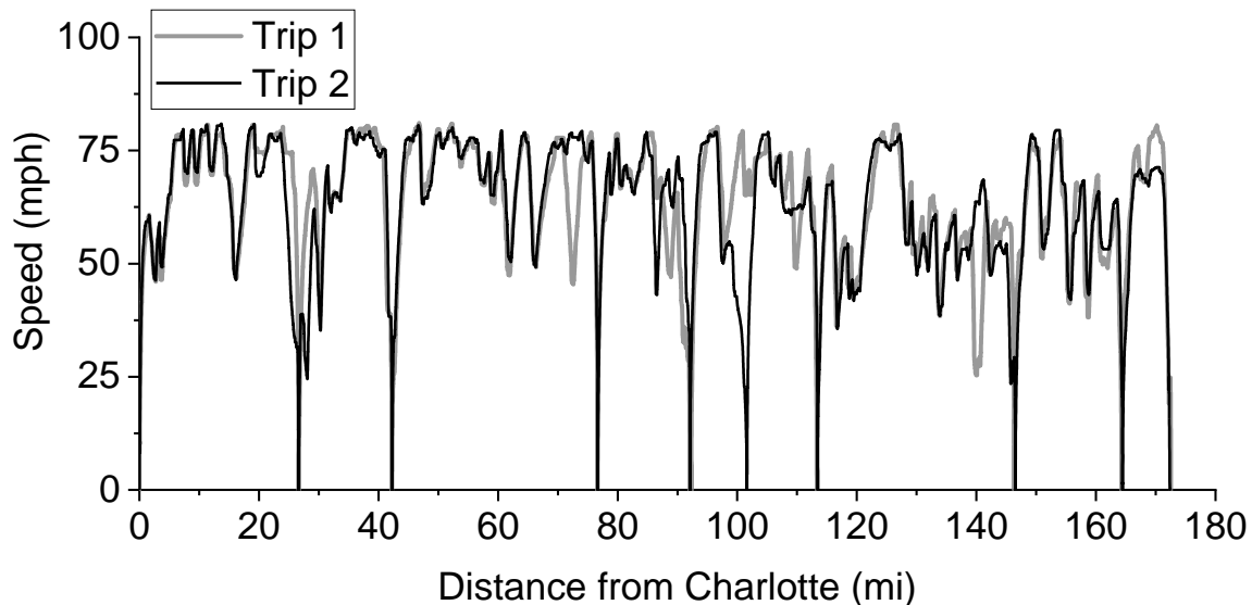
FIGURE 5-11. Variation in Speed with Distance for Two Selected One-way Trips Measured for Single Locomotive Consist of NC 1859 operated on ULSD from Charlotte to Raleigh, NC. Trip 1 had a duration of 12,643 seconds and Trip 2 had a duration of 13,137 seconds.
