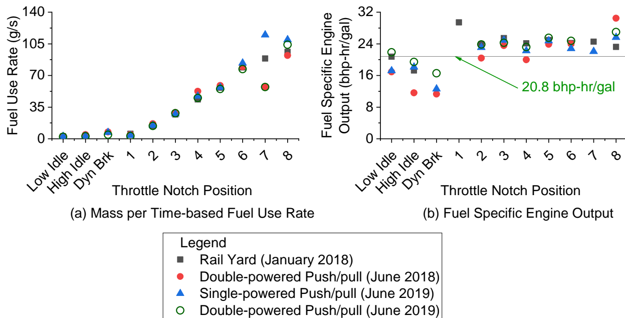
FIGURE 4-5. Comparison of Steady-State Notch-Average Fuel Use Rates for the Prime Mover Engine of Locomotive NC 1984 Between Rail Yard, Double- and Single-powered Push/Pull Over-the-Rail Measurements: (a) Mass per Time-based Fuel Use Rate; and (b) Fuel Specific Engine Output.
