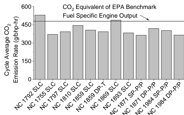
(a) Cycle-average CO 2 Emission Rates
